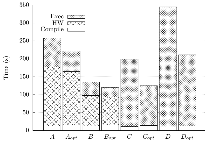
Figure 1: Benchmarks before and after optimisation.
